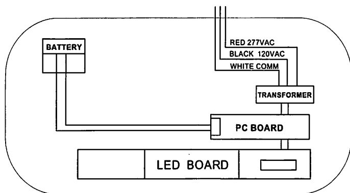
SELF DIAGNOSTIC WIRING DIAGRAM:
