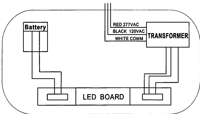
BATTERY BACKUP WIRING DIAGRAM:
