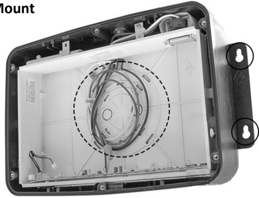
Ceiling Mount
